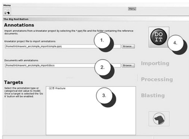
Figure 2 Screenshot of Automated Retrieval Consoles 'Do-It-Yourself' interface which allows non-technical end users to perform information retrieval in four steps: (1) annotated (Knowtator) project file selection; (2) document corpus selection; (3) select target or targets from those available in the list of annotations and; (4) launch the process.
